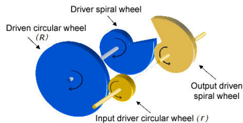
System Varistart (PH.B innovations)
